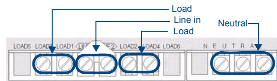
FIG. 2 High-voltage connections
